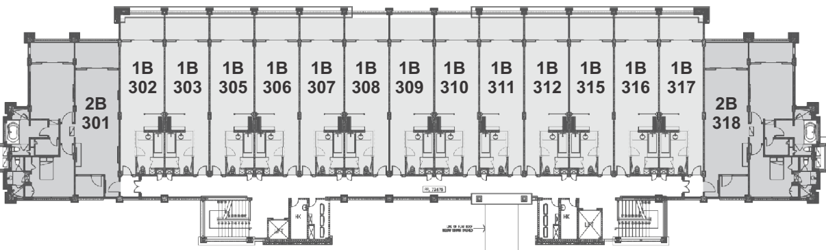
FIRST AND SECOND FLOOR PLAN
